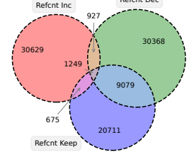
Figure 15: Refcount operations triggered in Linux v6.6 update refcount unidimensionally usually.
