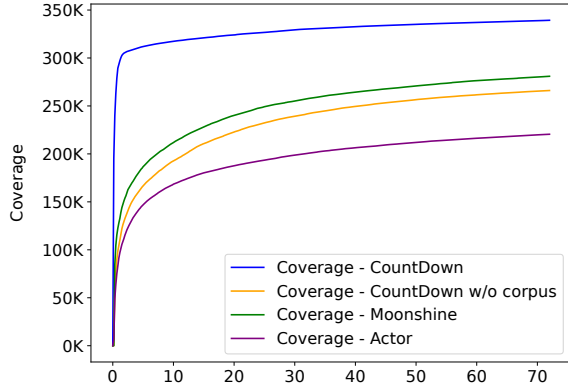
Figure 11: Coverage triggered by COUNTDOWN and advanced tools. Comparisons of any two tools are statistically significant ( p -values < 0.001 ).
